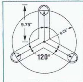
3-Way 120° Tie Brace
