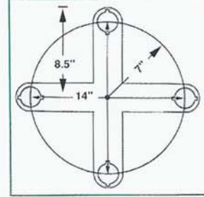
4-Way Tie Brace
