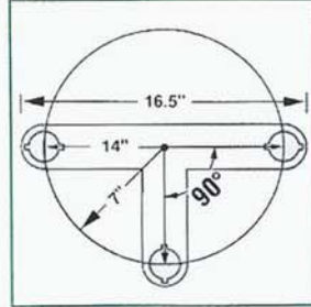
3-Way 90° Tie Brace
